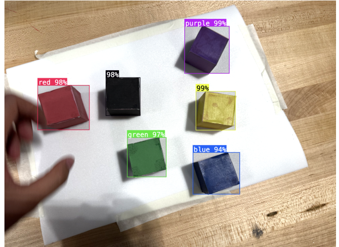
Fig. 4. A sample detection and classification result from our trained YOLO model. Each block is correctly detected and its color correctly inferred; prediction confidence (in percent) is shown above each bounding box.
